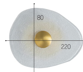
하림 B/R SIZE W220×D75×H80mm LAMP LED 3W, 3000K 후렌지 W120×D120×H30mm
