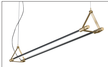
LED hexa 2등 P/D SIZE W1095×D115×H115 LAMP LED 38W (4000K)
